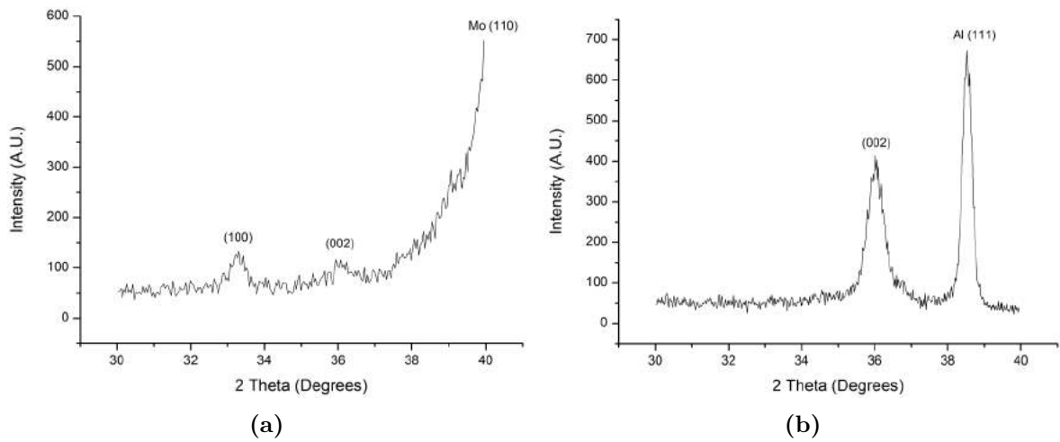
Figure 5.8: XRD results for a grazing incidence approach, scans were performed from 30^\circ to 40^\circ , both figures taken from [83] a) wafer 9. b) wafer 10.
