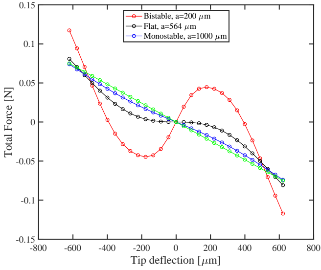
Fig. 6. Total force respect to tip deflection for monostable, bistable and flat potential cases. The NS configuration was considered and for all cases b = 500 \mu\text{m} .
