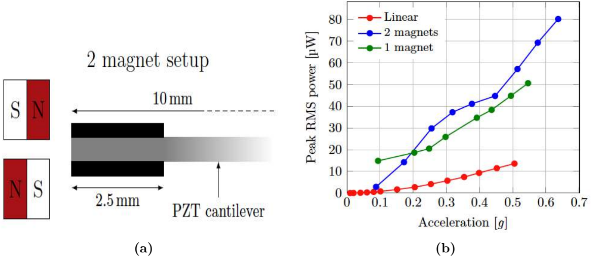
Figure 1.11: Magnetic system proposed by Lei et al., taken from [17]. a) Set-up b) RMS power harvested in the linear regime versus the non-linear regimes.
