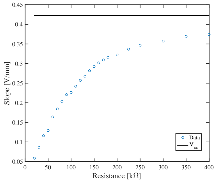
Figure 7.33: The slope of every line in the previous figure is taken as each of them represents a point in this plot. The horizontal black line represents the open circuit voltage slope.
