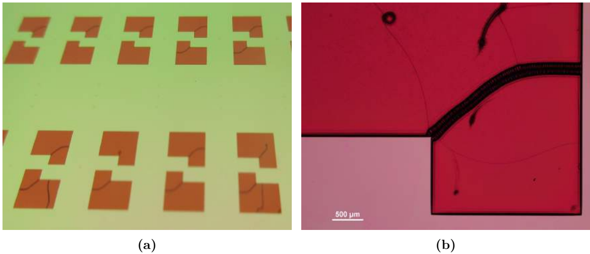
Figure 5.18: Wafer with cracks developed on the resist after ≈ 10 min of etching in AR under the conditions described in Table 5.5. a) Regular picture b) Microscope picture.
