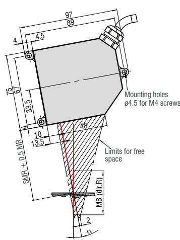
optoNCDT 2300-2 ... 2300-20 Direct reflection
