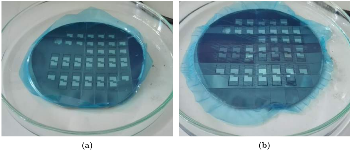
Figure 6.11: Procedure followed to detach the beams from the electrostatic tape. a) The wafer is dipped in a petridish filled with acetone. b) After a minute inside the petridish the tape starts to detach and some curls are formed.
