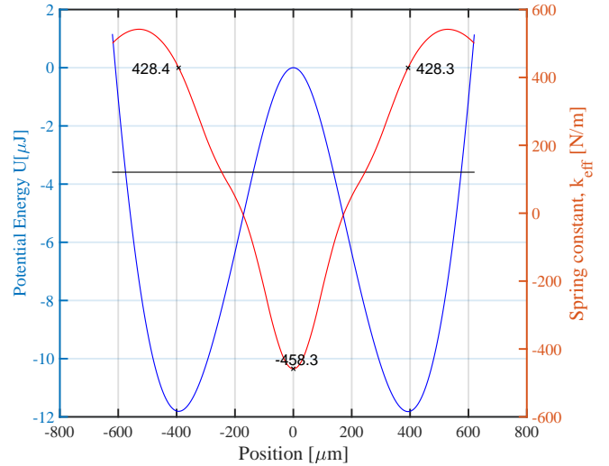
Fig. 8. k_{\text{eff}} and total potential energy associated to the bistable case ( a = 200 \mu\text{m} and b = 500 \mu\text{m} ) for the NS configuration. The black line represents the spring constant associated to the linear case
