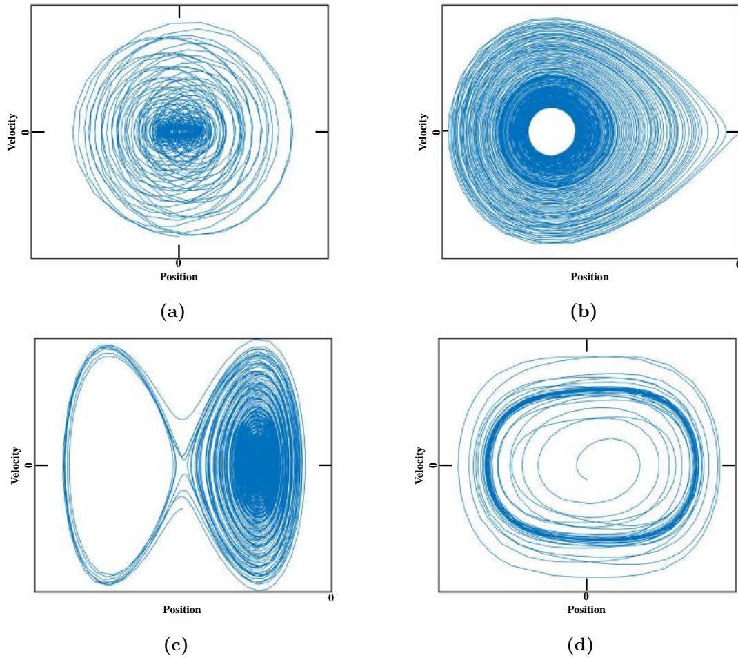
Figure 3.3: Different position-velocity phases that correspond to four different dynamics. a) Mono-stable, the beam oscillates around zero tip deflection with small amplitude oscillations. b) Bi-stable with small amplitude oscillations around one of the stable positions, i.e. around one of the magnets. c) Bi-stable with large amplitude oscillations in the beginning whereas in the end the beams is confined to one well. d) Flat potential landscape, the beam performs large amplitude oscillations.
