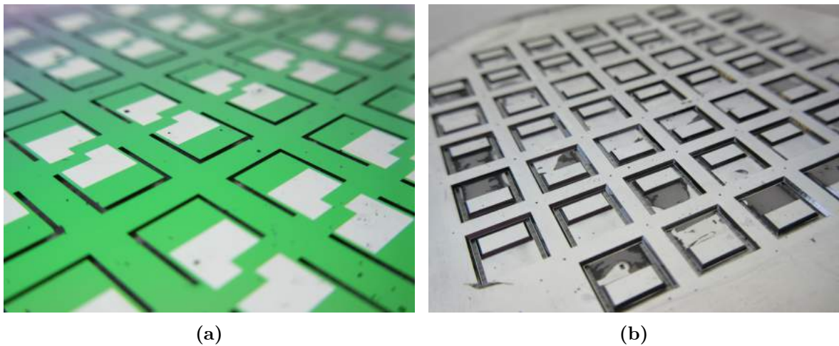
Figure 6.9: Final devices before being diced out. (a) Front side view. (b) Backside view.
